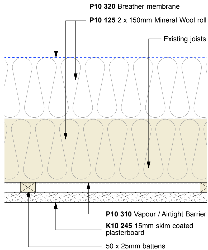
2 Pitched roof - insulation at ceiling level Scale: 1:5
