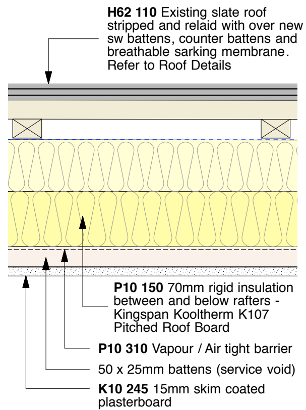
1 Pitched roof - insulation between rafters Scale: 1:5
