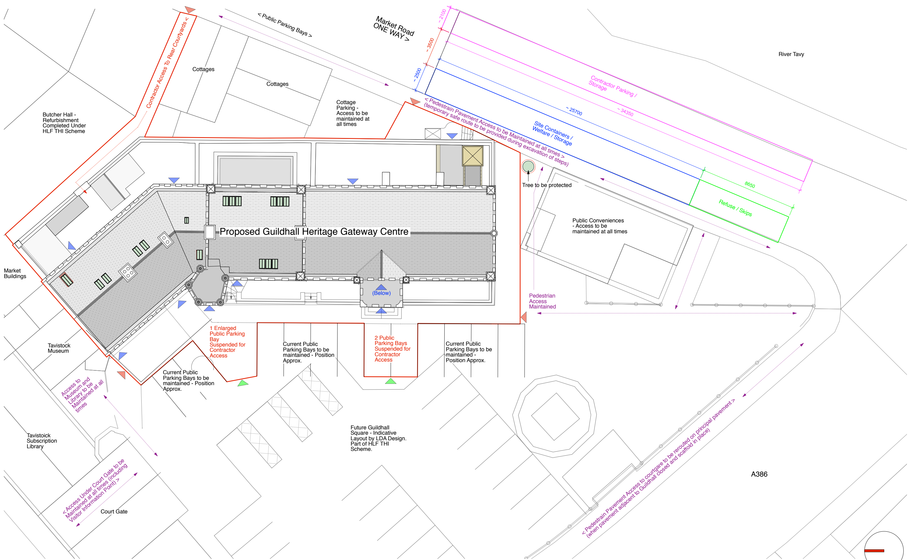
tavistock guildhall TTC Construction Site Constraints Plan as Proposed - 1:100 @ A1 - NOTE: FINAL LAYOUT TO BE PROPOSED BY CONTRACTOR AND AGREED WITH CLIENT
